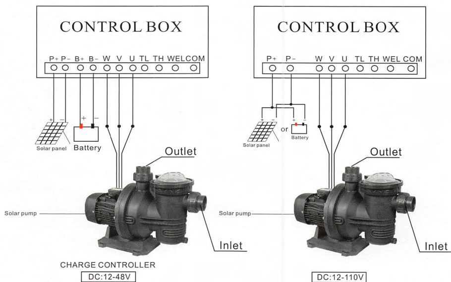
internal wiring diagram
